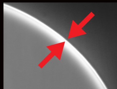
素材:鉄粉(平均粒径:10μm) Substrate: iron powder with an average particle diameter of 10μm 膜厚:約100nm Thickness: About 100nm
