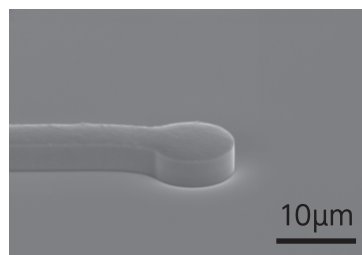
Current density 1.0 A/dm 2 , surface thickness 5 µm
