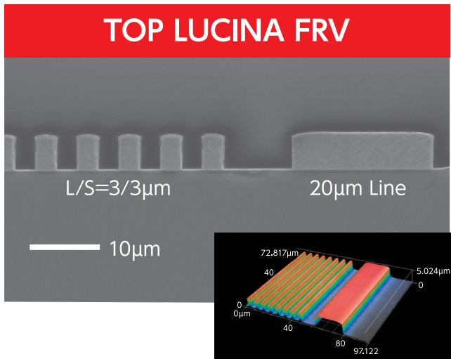
Current density 1.0 A/dm 2 , surface thickness 5 µm
