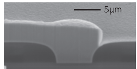
Current density 1.0 A/dm 2 , surface thickness 5 µm
